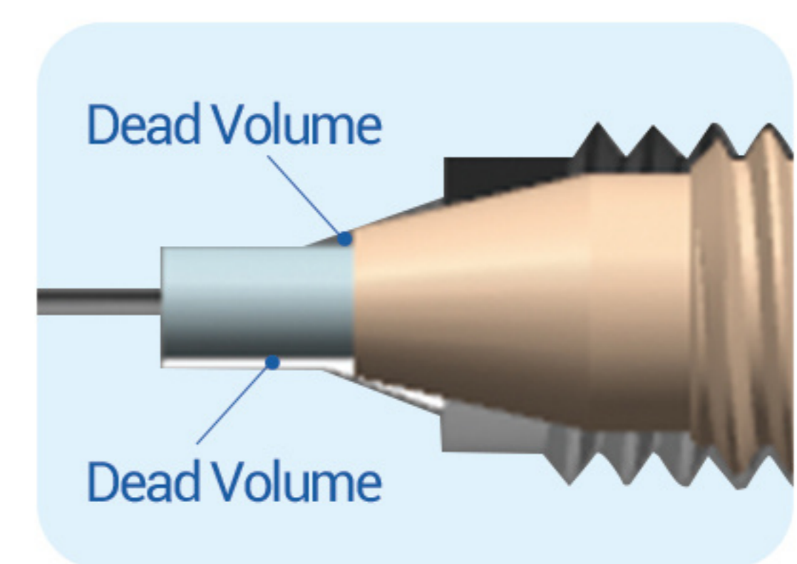
Dead Volume Position of Regular Fitting
